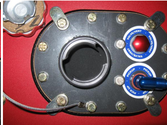
RUBBER "FLAP" INSIDE THE FILL NECK
